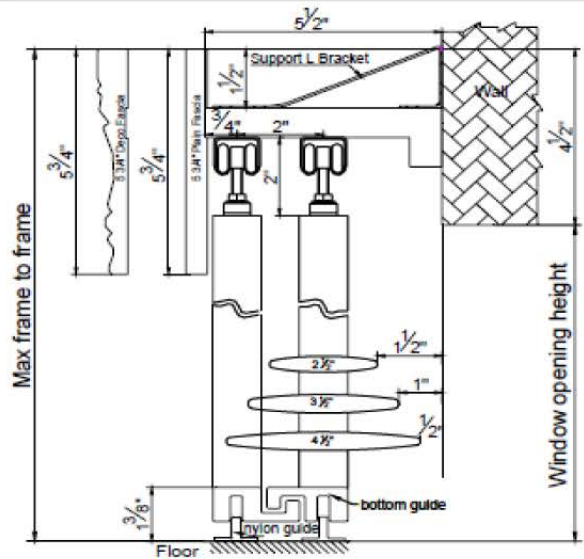
By-pass Track Single Panel Specs
